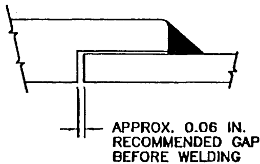
Figure 2 - Welding Gap
